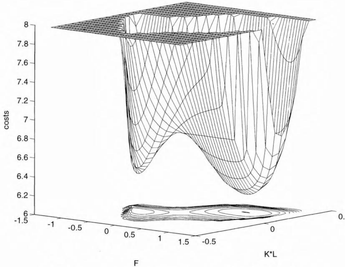
Fig. 1. Local optimality, n_x = 10 , n_u = n_y = 1 , \text{srp} = 0.95 , \text{seed} = 89 (see Appendix 2).
