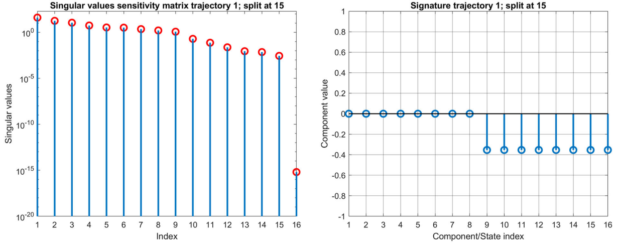
Figure 4. Singular values indicating a single numerically zero singular value and corresponding unobservable mode (left panel). From the observability signature (right panel), the single unobservable mode is a combination of state-variables 9–16 being all phases \phi_i , i = 1, 2, \dots, 8 of all oscillators. The CPU-time on an ordinary Windows 10 PC was 2.62 s.
