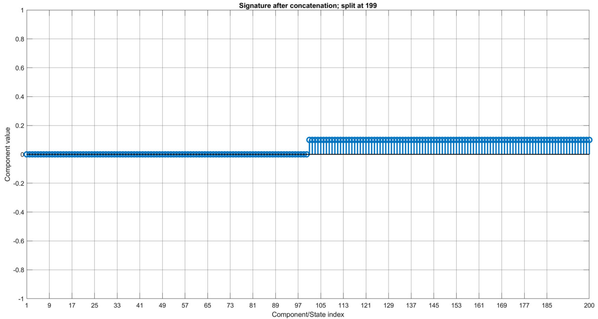
Figure 6. Observability signature for the system containing one hundred oscillators showing that the single unobservable mode is a combination of all phases x_{i+100} = \phi_i, i = 1, 2, \dots, 100 being the last one hundred state-variables.
