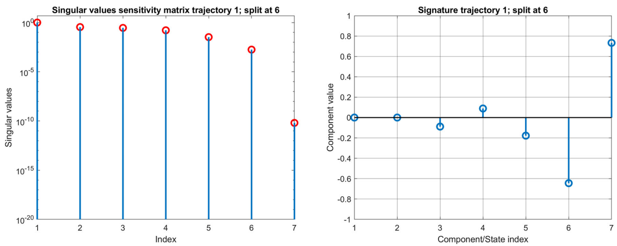
Figure 2. Singular values and controllability signature of the CSTR with three control variables as obtained from the sensitivity-based algorithm. The left panel shows one numerically zero singular value corresponding to a single uncontrollable mode. The right panel shows the corresponding controllability signature indicating that the single uncontrollable mode is a combination of state-variables 3–7.
