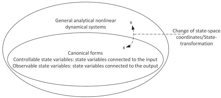
Figure 1. Canonical forms facilitating simple definitions/explanations of controllability and observability as connectivity's to the input and output. Changes of coordinates/state-transformations connect analytical nonlinear dynamical systems to their canonical forms.
