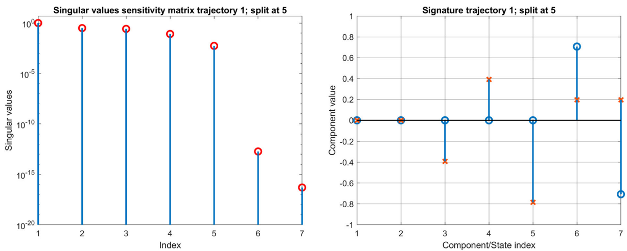
Figure 3. Singular values and controllability signature of the CSTR with two control variables as obtained from the sensitivity-based algorithm. The left panel shows two numerically zero singular values corresponding to two uncontrollable modes. The right panel shows the corresponding controllability signature indicating that the two uncontrollable modes involve state-variables 3–7.
