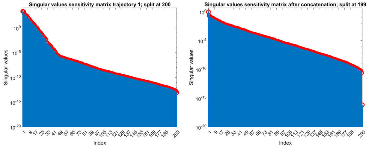
Figure 5. Two hundred singular values obtained from the sensitivity-based algorithm for one trajectory (left panel) and when concatenating the result of six trajectories (right panel). Only the latter correctly shows a single numerically zero singular value and corresponding unobservable mode. Each trajectory started from the same initial condition and had a final time 10, but used different values for the two parameters \alpha, \beta . The total CPU time on an ordinary Windows 10 PC to compute all six trajectories was 364 s.
